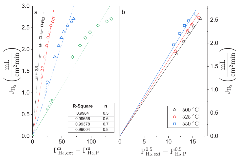
Fig. 5. (a) H_2 permeation flux at T = 500 °C for several values of n . (b) Effect of temperature on the H_2 permeation flux through a Pd-Ag membrane. In both cases P_{H_2,ext} \approx (P_{H_2,F} - P_{H_2,R}) / \log(P_{H_2,F}/P_{H_2,R}) .
