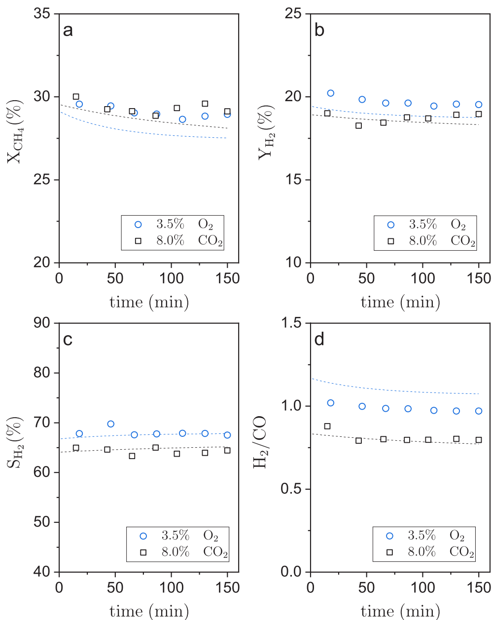
Fig. 10. Effect of using O 2 or CO 2 as regenerating gas in a TZFBR. (a) CH 4 conversion. (b) Yield of H 2 . (c) Selectivity to H 2 . (d) H 2 /CO molar ratio. T = 525 °C. W = 30 g, u r = 3. W = 30 g. Experimental data (symbols), model prediction (lines).
